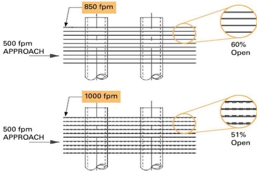
Plan View Drawing of Coils
